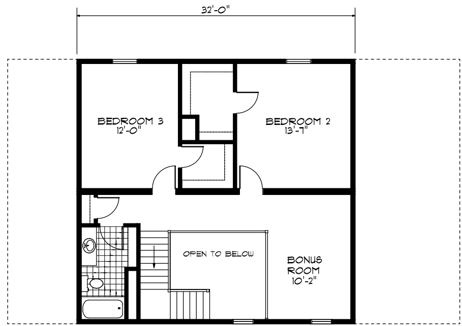
SECOND FLOOR 981 SQ. FT.
